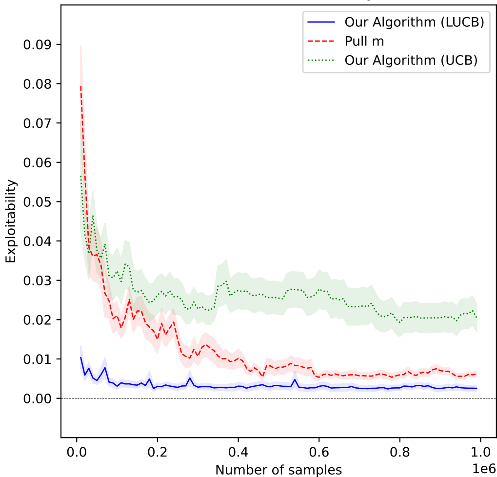
Leduc Poker, Variations, Player x
